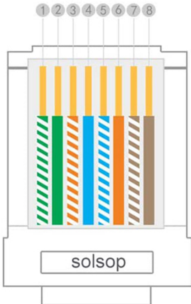
T568A Standard
