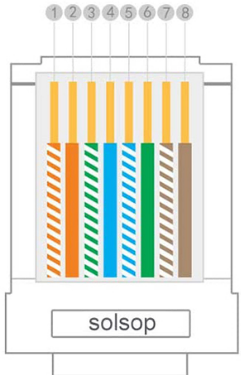
T568B Standard
